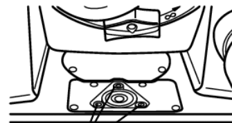
Circular vial adj. screw
